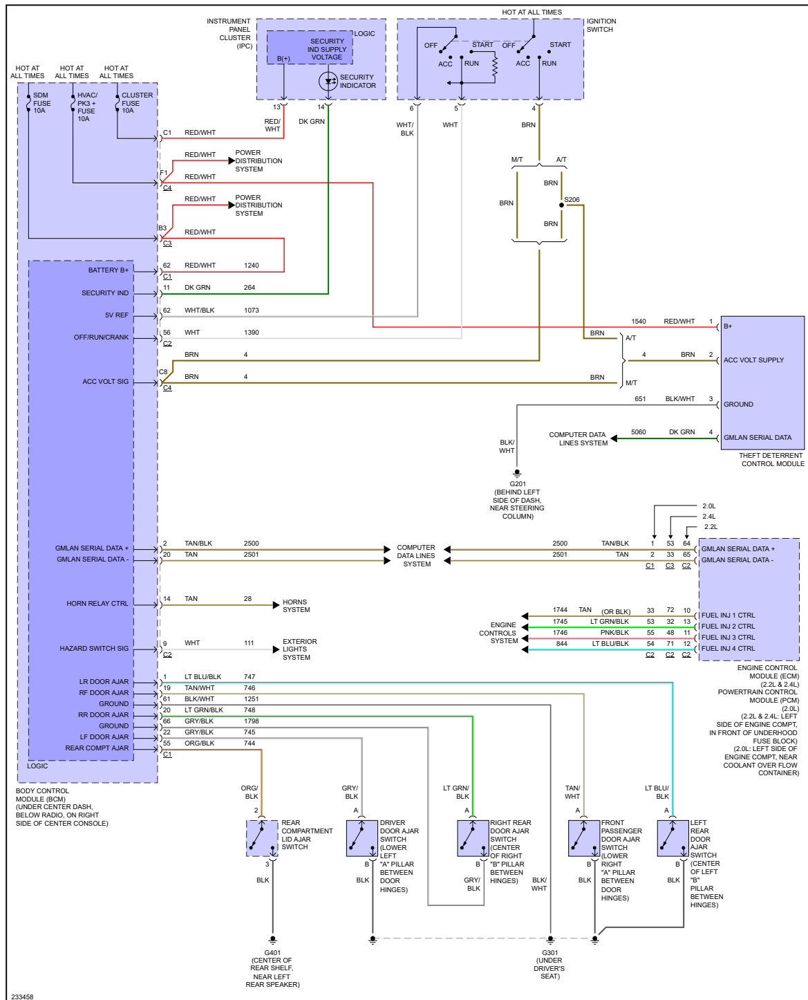
Fig 1: Anti-theft Circuit
