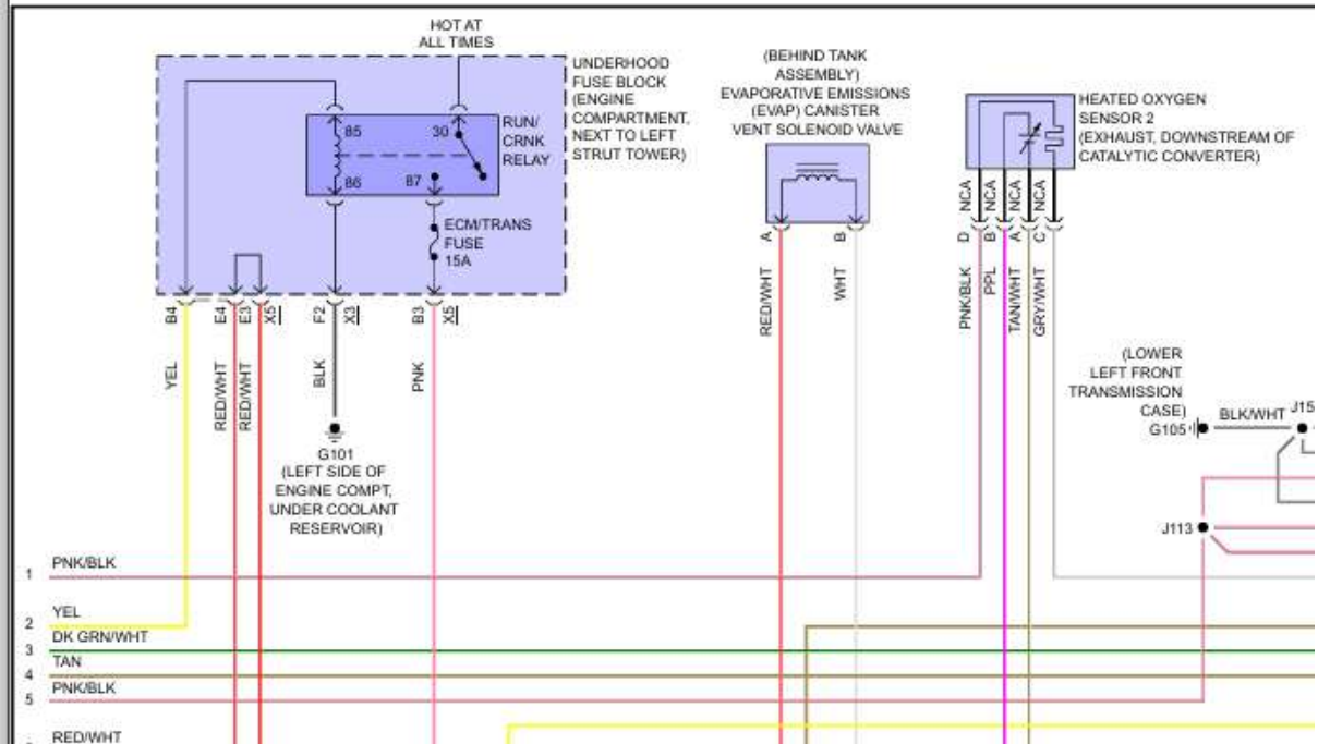
Fig 4: 2.0L VIN X, Engine Performance Circuit (4
