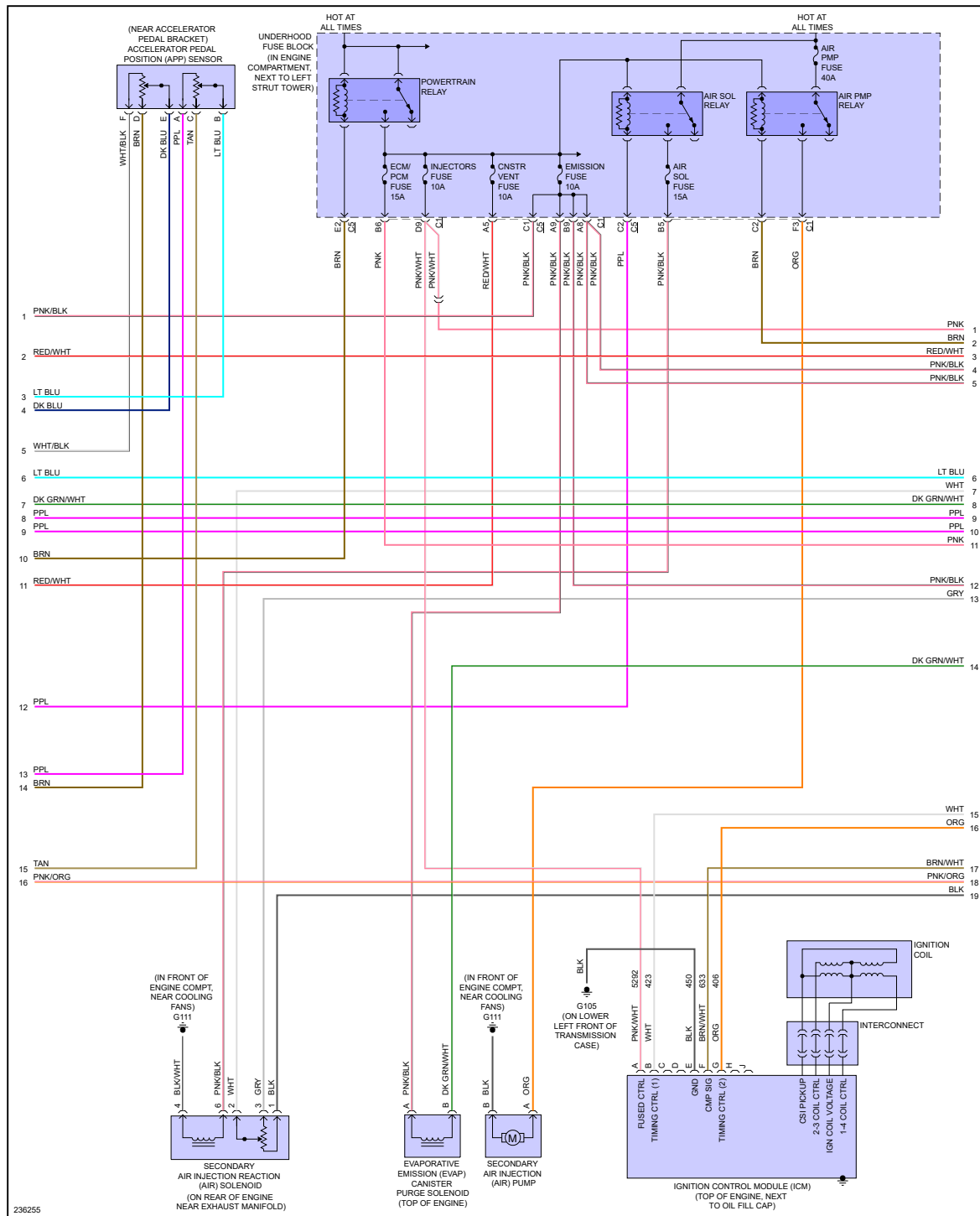
Fig 2: 2.2L VIN F, Engine Performance Circuit (2 of 4)
