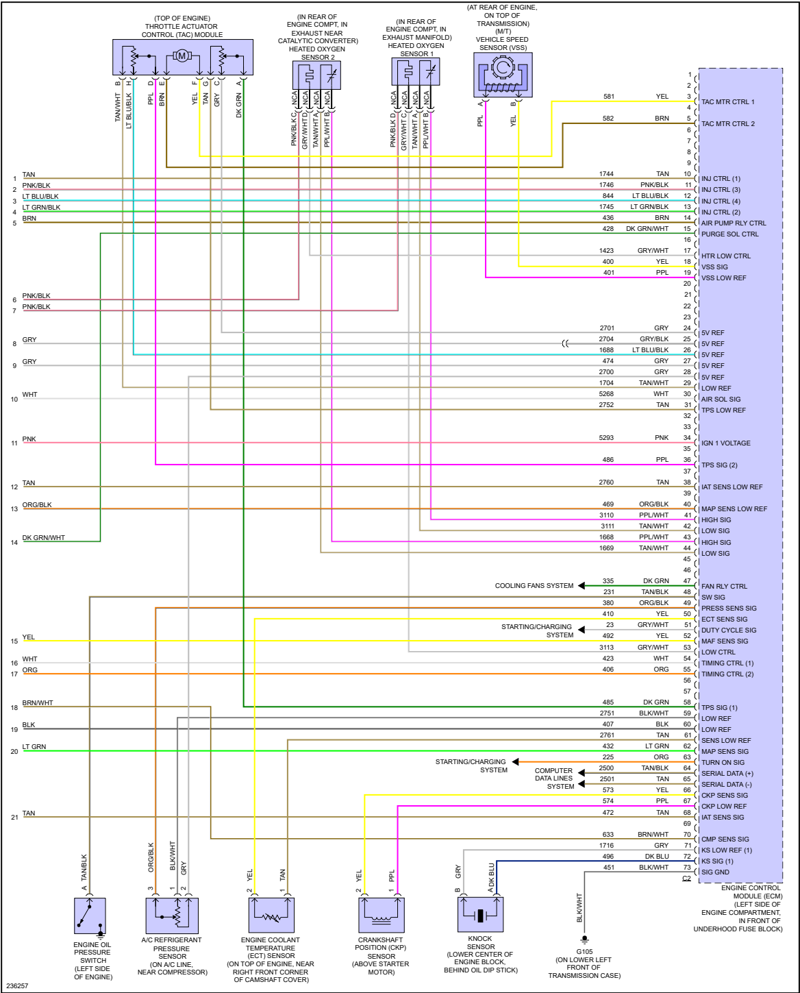
Fig 4: 2.2L VIN F, Engine Performance Circuit (4 of 4)
