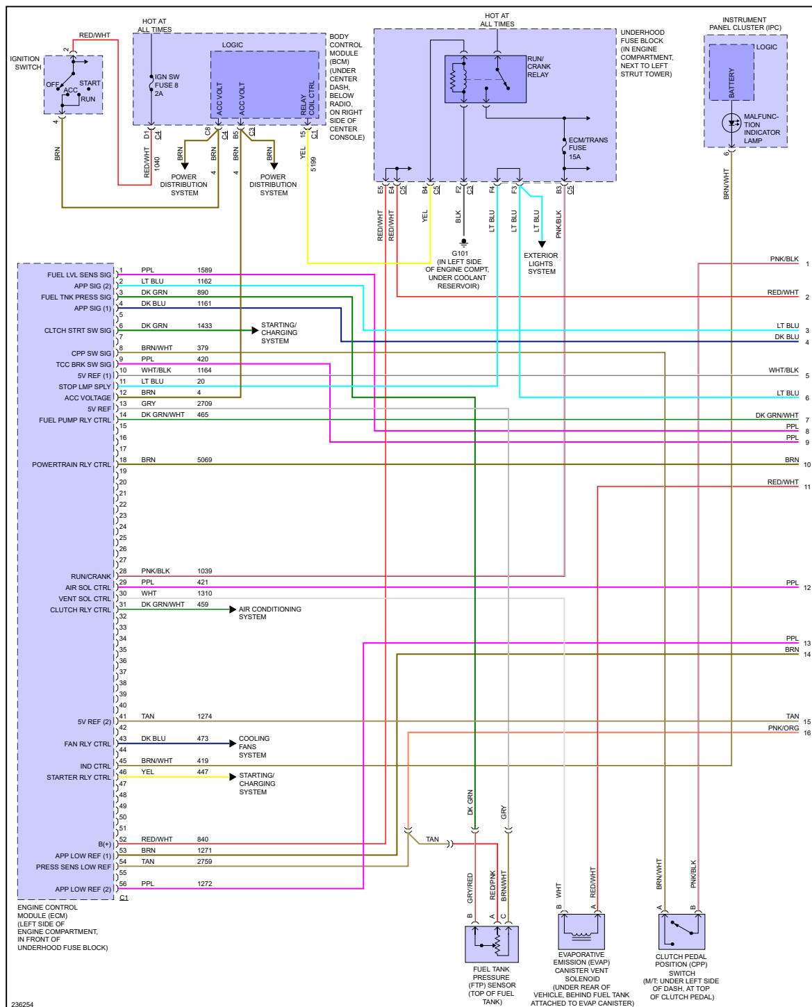
Fig 1: 2.2L VIN F, Engine Performance Circuit (1 of 4)
