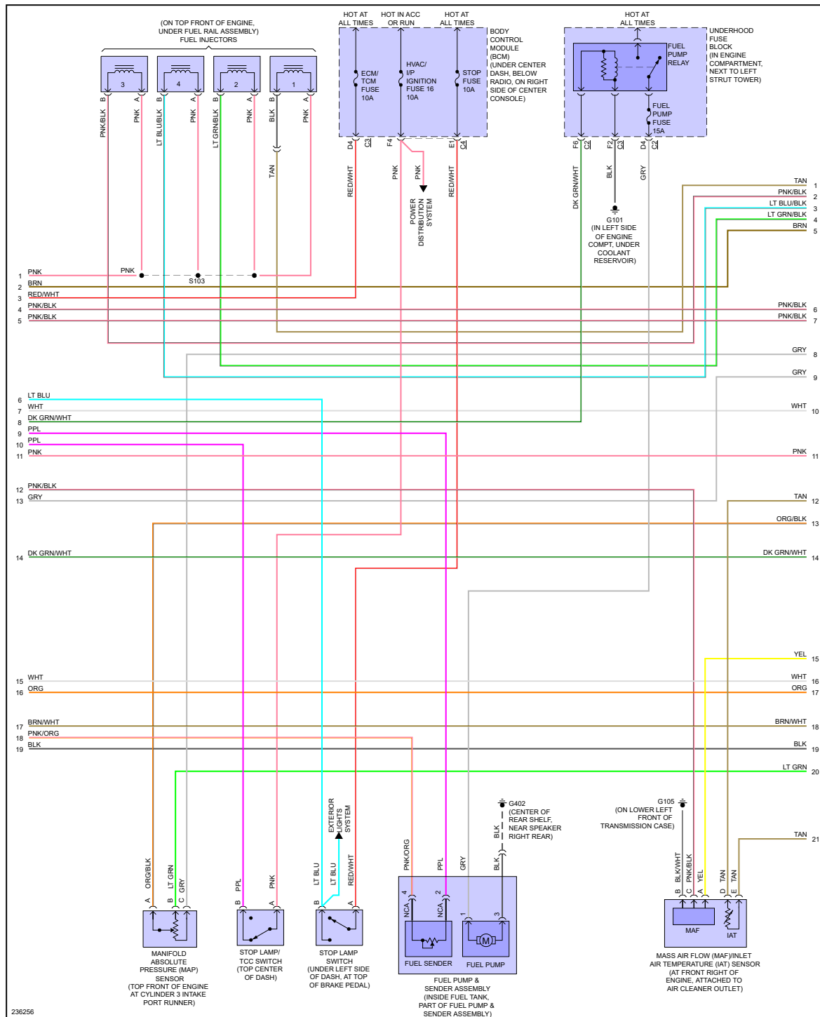
Fig 3: 2.2L VIN F, Engine Performance Circuit (3 of 4)
