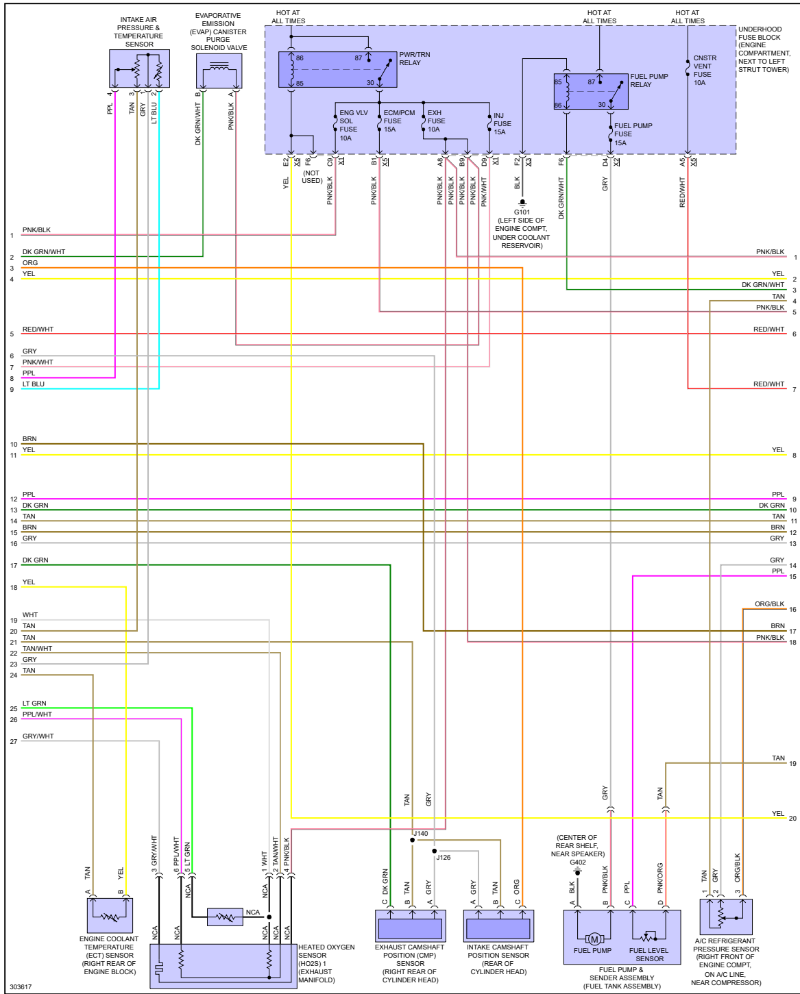
Fig 3: 2.0L VIN X, Engine Performance Circuit (3 of 4)
