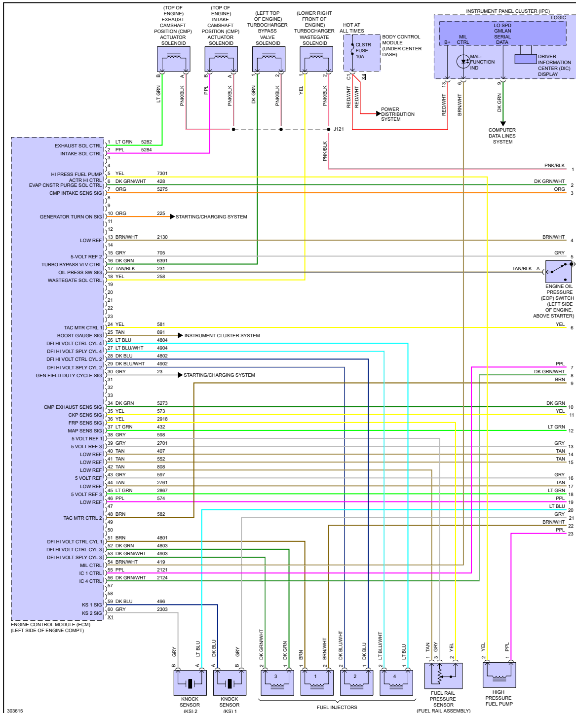
Fig 1: 2.0L VIN X, Engine Performance Circuit (1 of 4)
