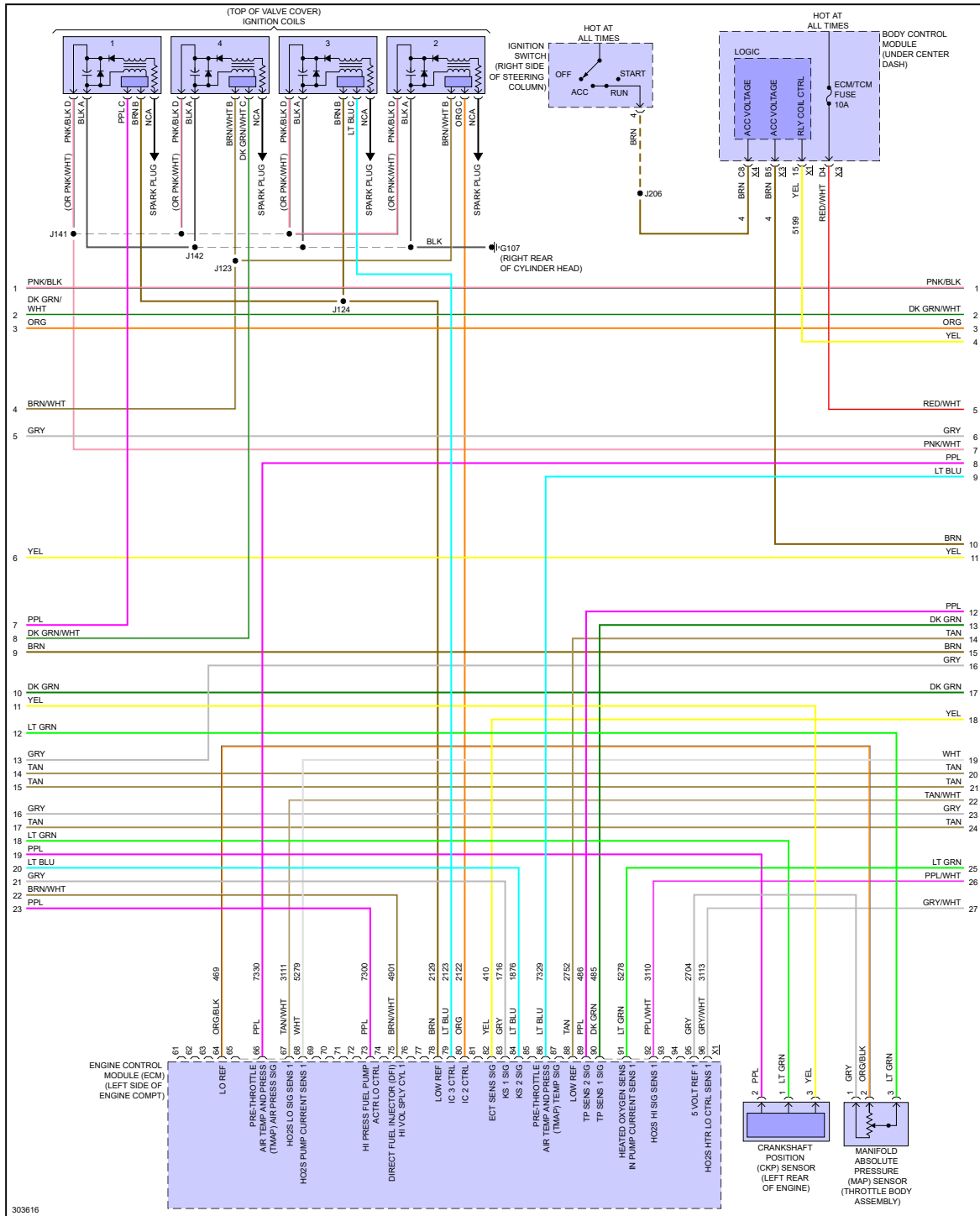
Fig 2: 2.0L VIN X, Engine Performance Circuit (2 of 4)
