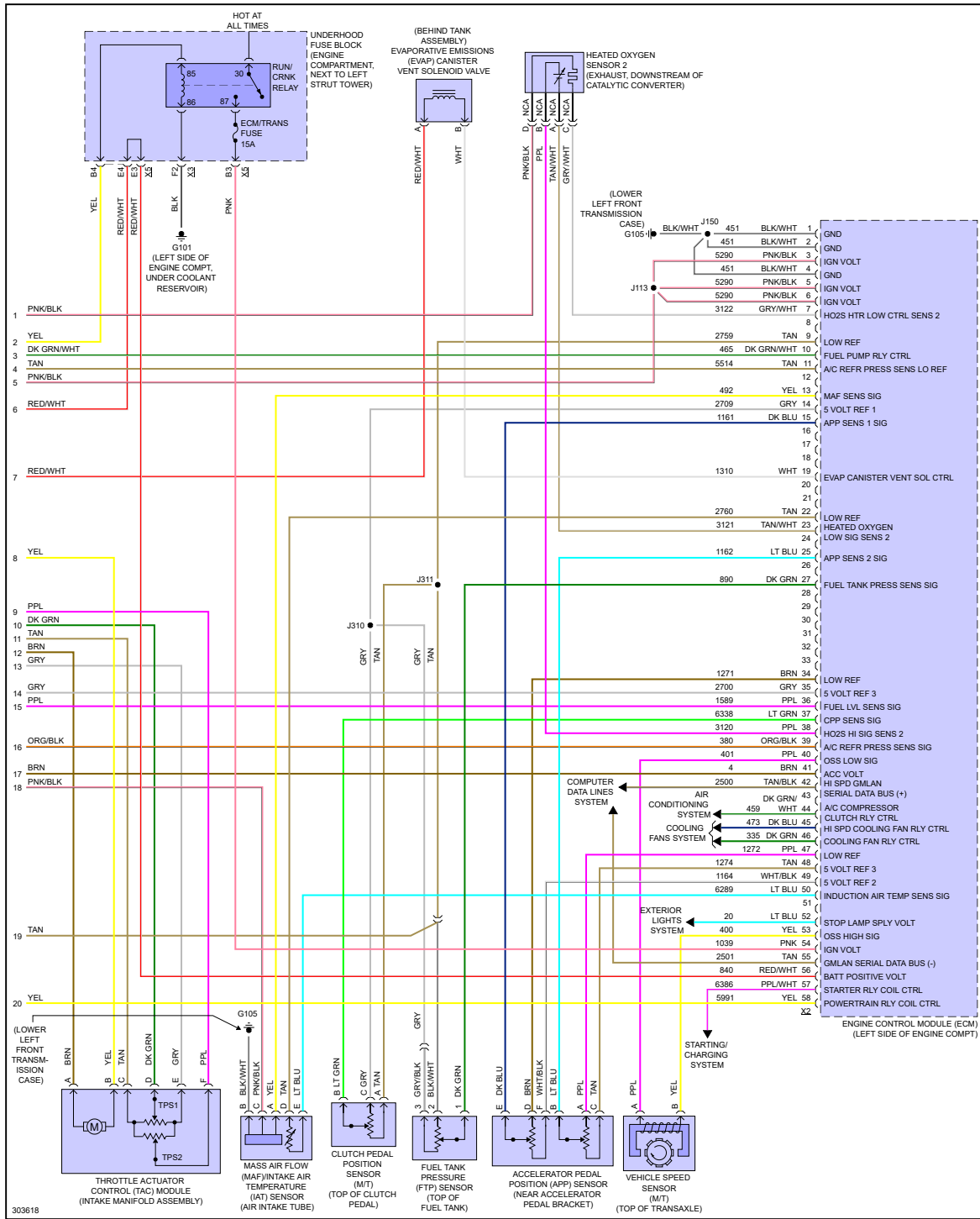
Fig 4: 2.0L VIN X, Engine Performance Circuit (4 of 4)
