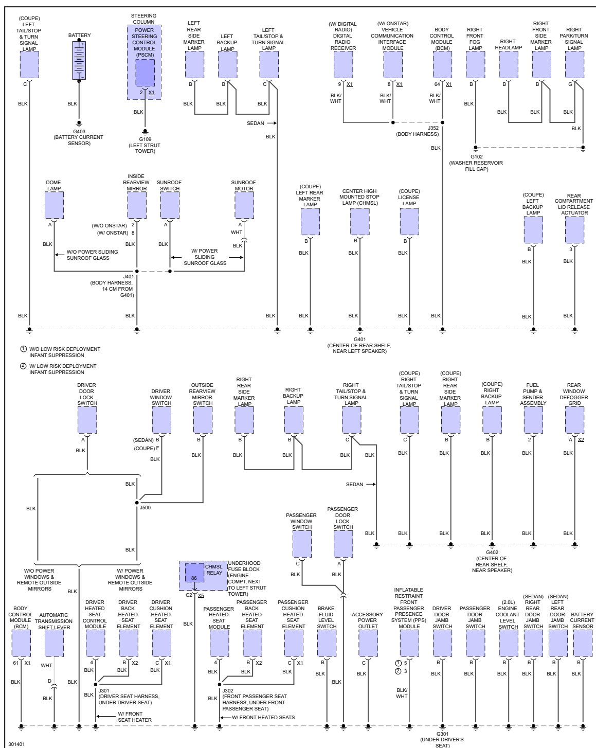
Fig 2: Ground Distribution Circuit (2 of 2)
