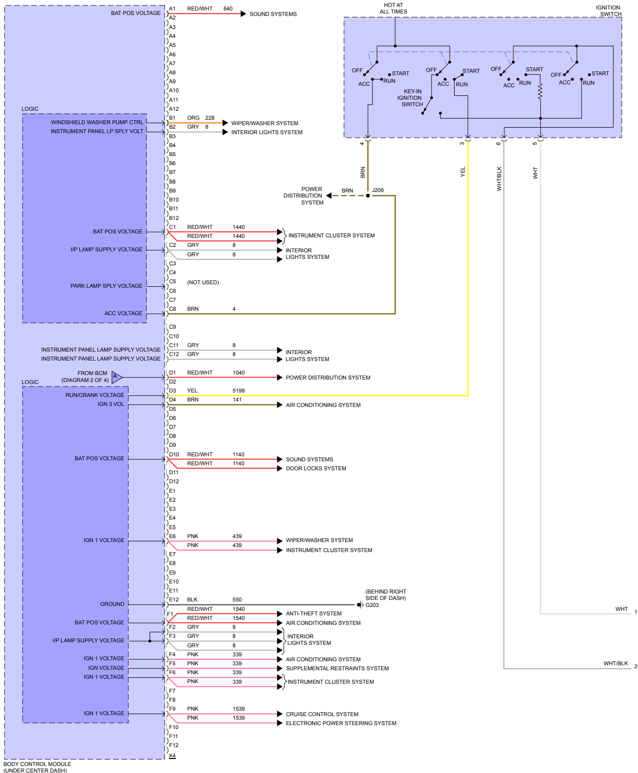
Fig 3: Body Control Modules Circuit (3 of 4)
