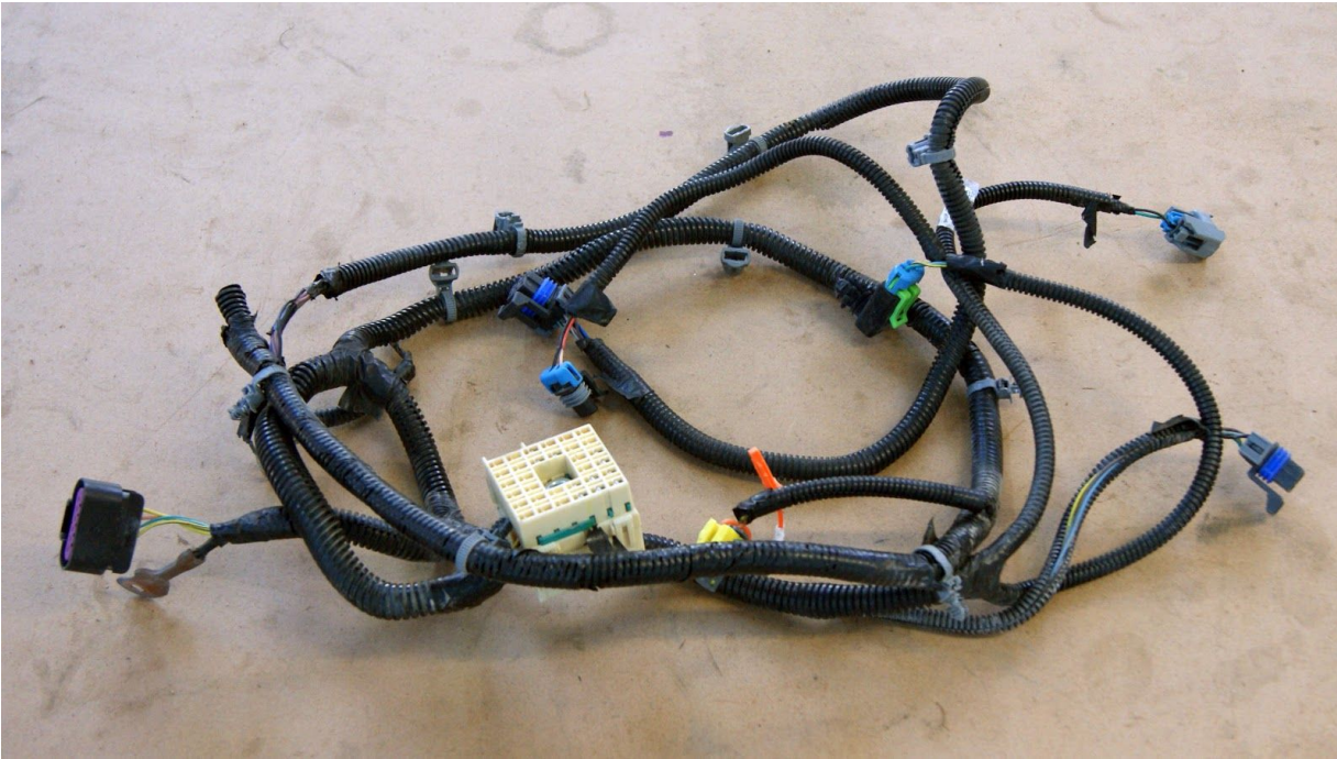
Headlight Harness
